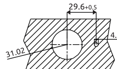
ASSEMBLY
