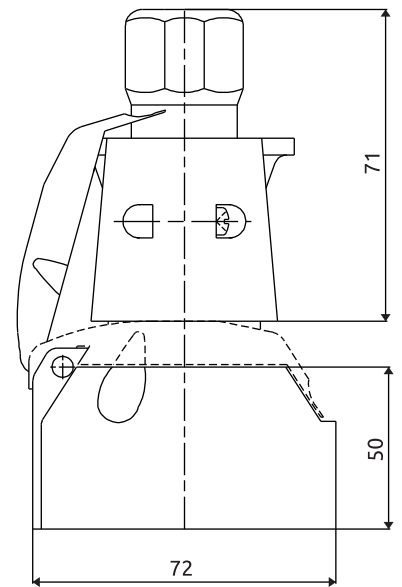
Cable Assembly
